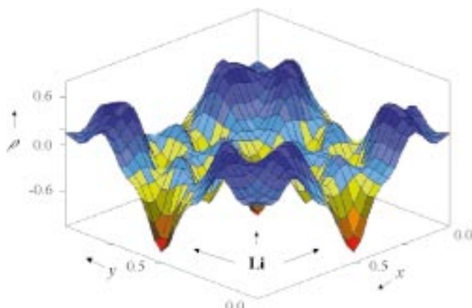
Figure 2. Difference Fourier map for z=0 showing the location of Li atoms at (1/2, 0, 0) and equivalent positions. The vertical axis corresponds to the scattering density \rho (in \text{fm } \text{\AA}^{-3} ), which is negative at the Li positions.
